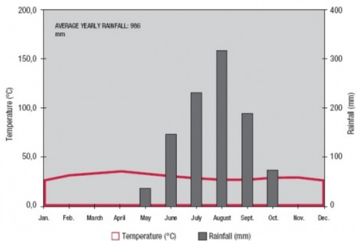
Figure 3. Climatic diagram of Kita
