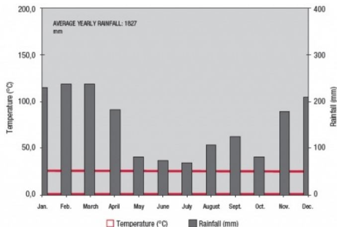
27 Figure 5. Climatic diagram of Savannakhet
