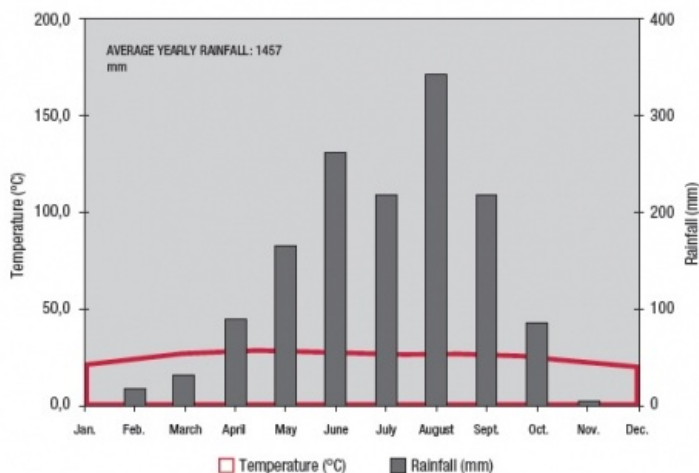
27 Figure 5. Climatic diagram of Savannakhet
