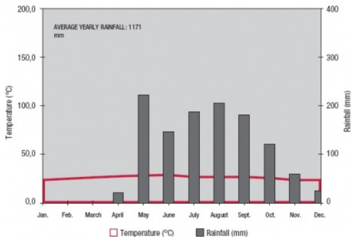
Figure 2. Climatic diagram of Binh Thuan
